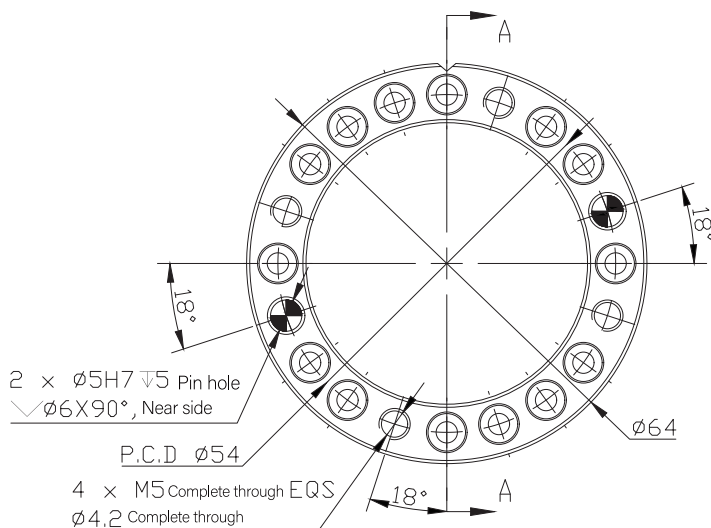
End flange installation dimensions
