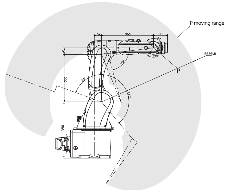
P moving range
