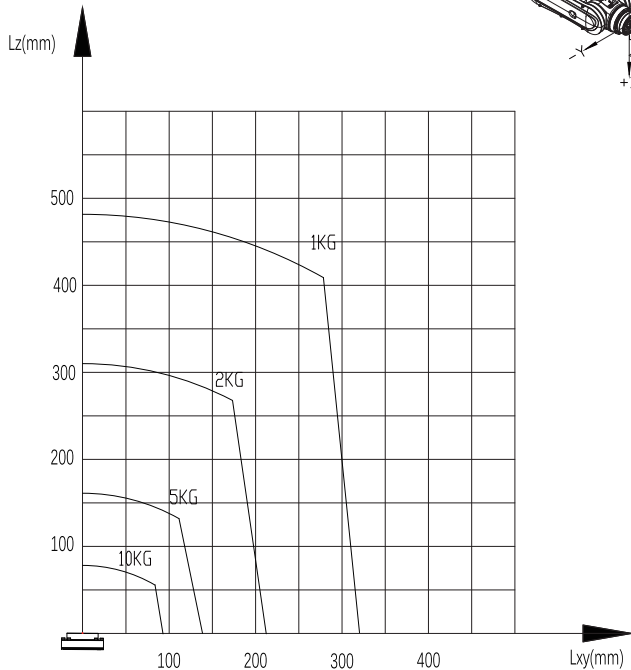
Robot payload diagram
